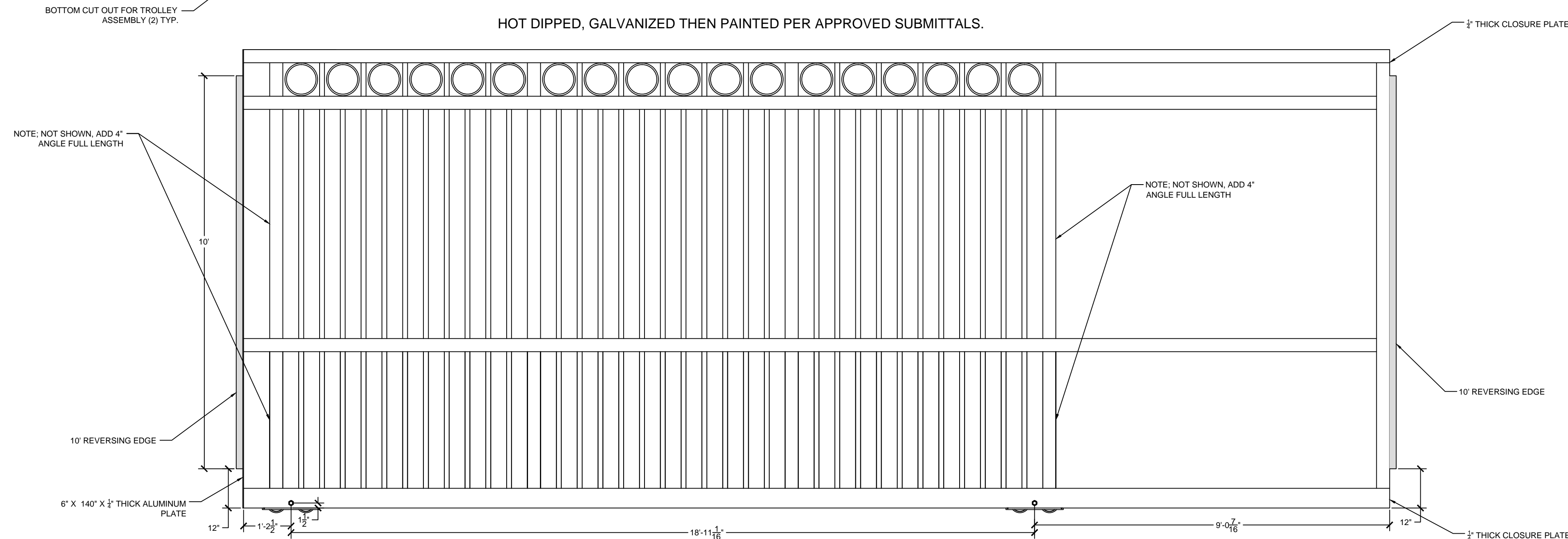
VEHICLE GATE FRAMING DETAILS
