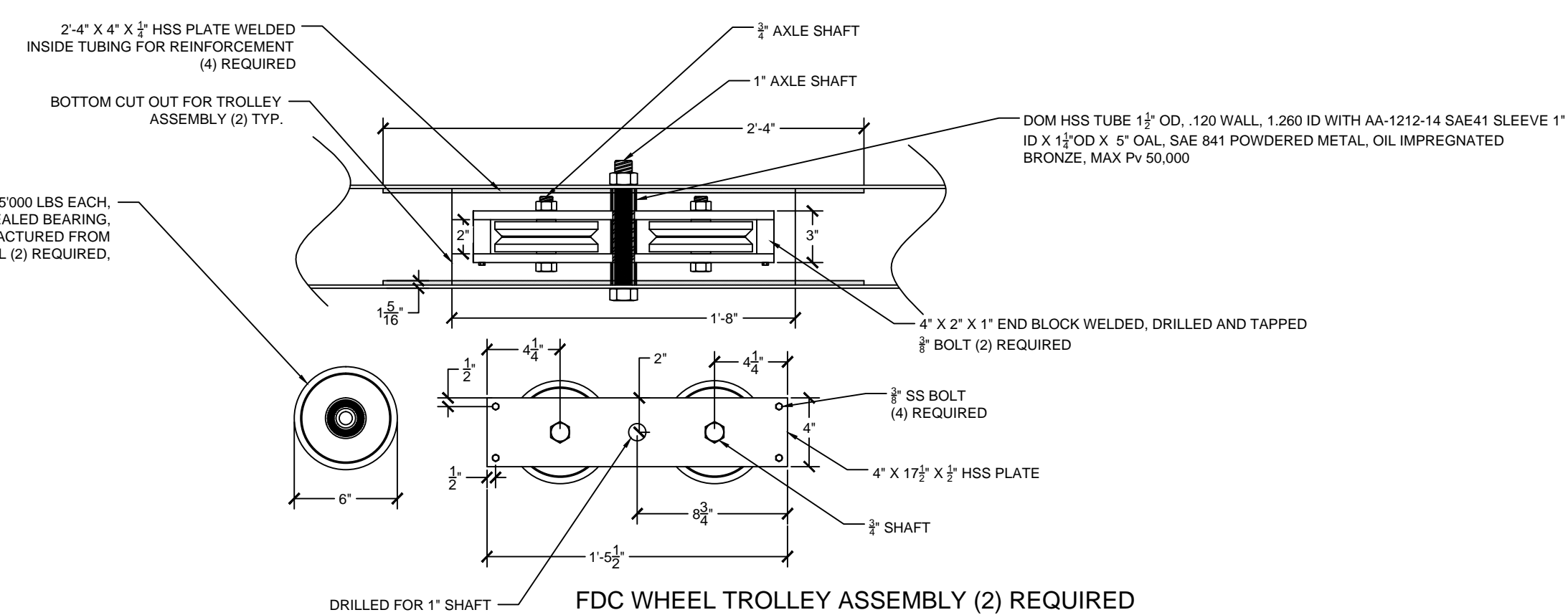
FDC WHEEL TROLLEY ASSEMBLY (2) REQUIRED
