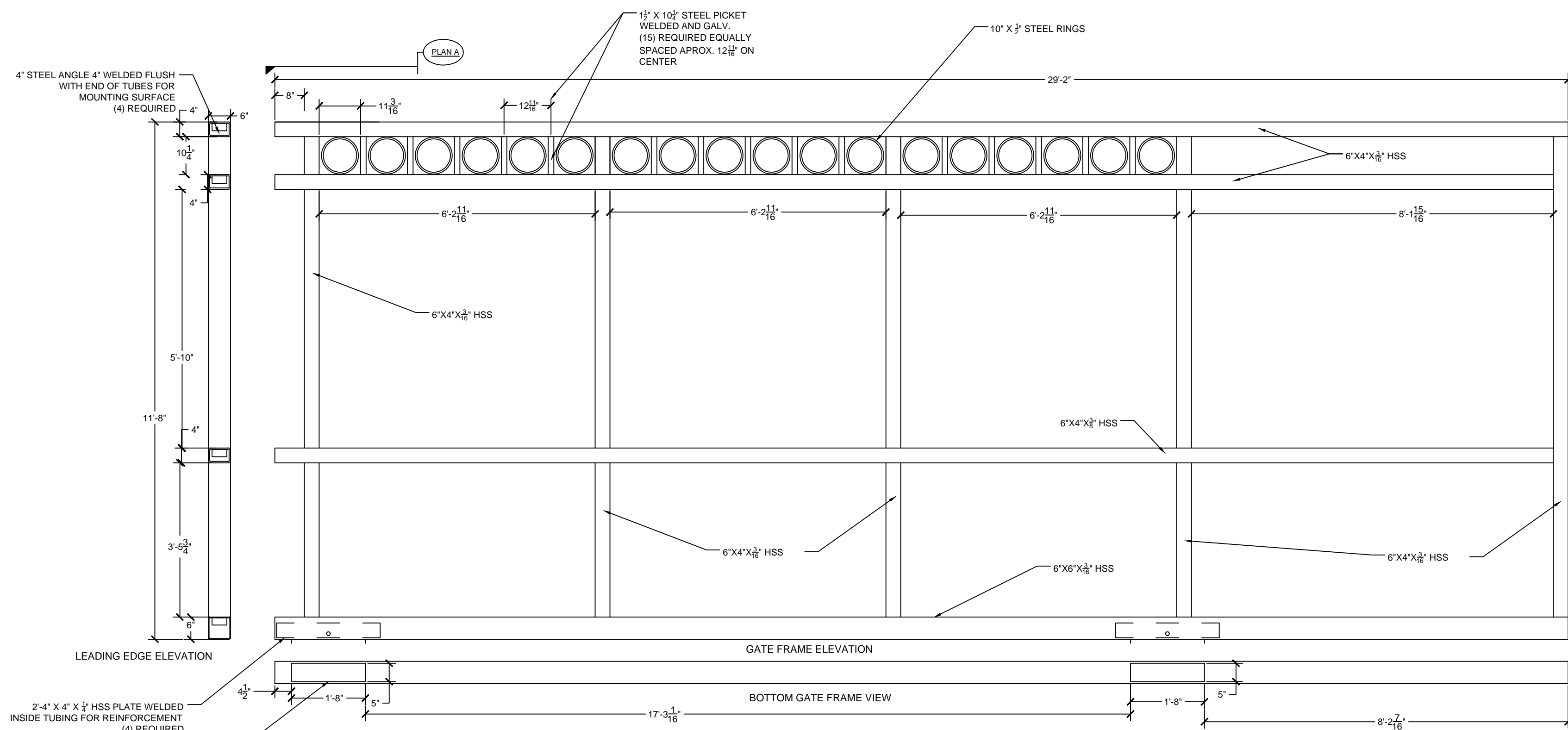
VEHICLE GATE FRAMING DETAILS
