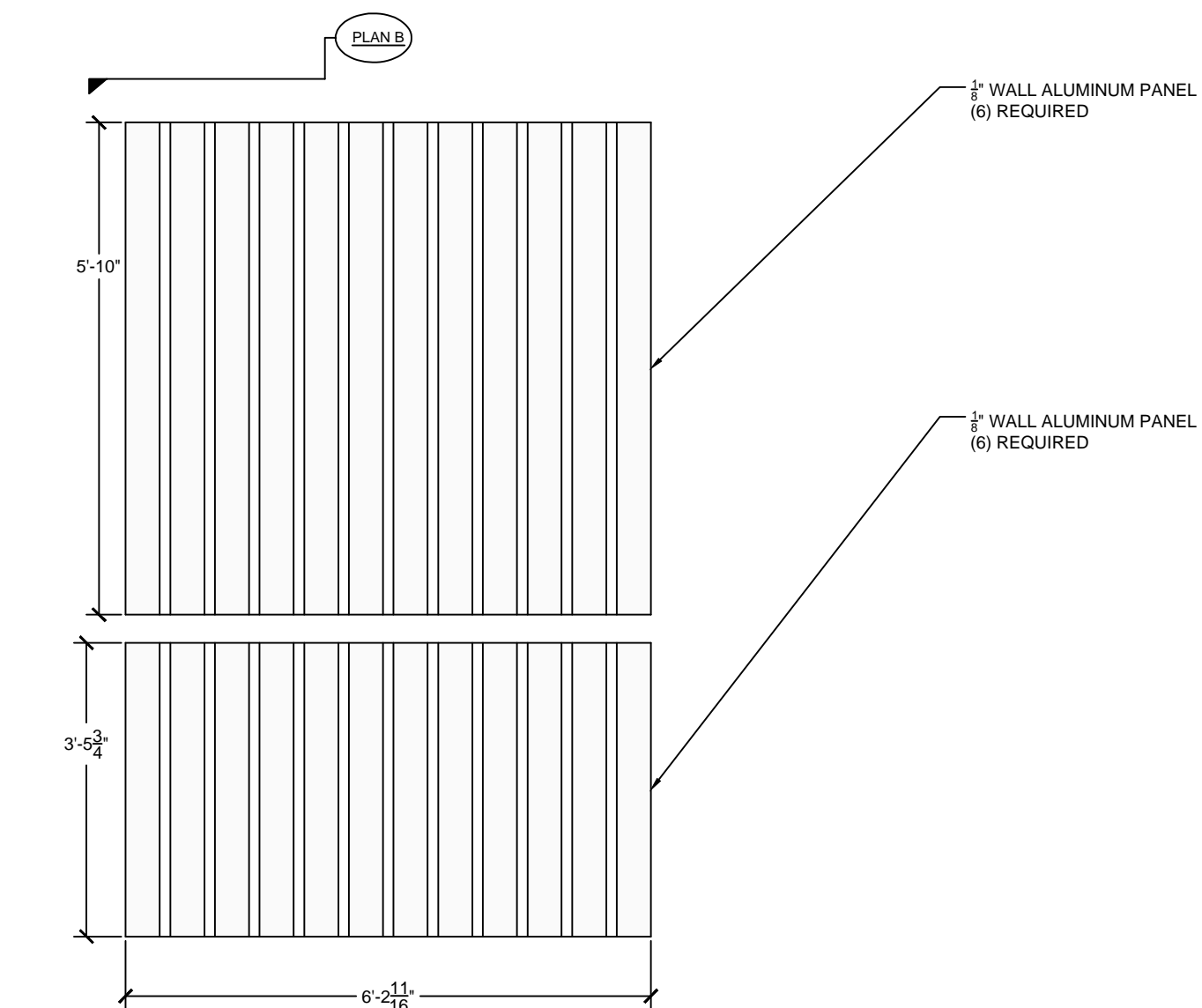
VEHICLE GATE FRAMING PANEL DETAILS
