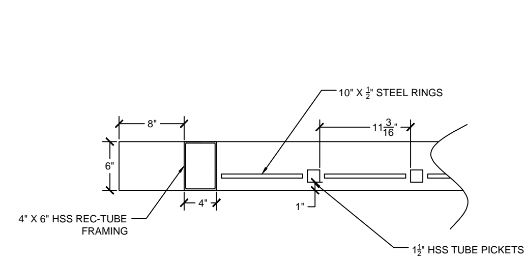
VEHICLE GATE OPEN RING DETAIL, PLAN (A)
