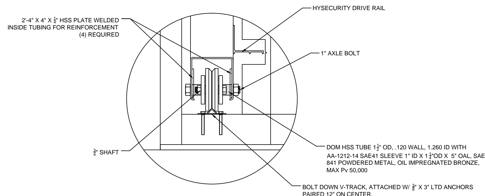
TROLLEY ASSEMBLY ELEVATION DETAILS
